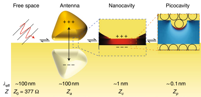
Fig. 1 | Impedance matched coupling of light from free space to atomic scale. Schematic of cascade of effective wavelength scales between free-space photons, coupled via antennas into nanogap modes, which can then couple to atomic-scale protrusions ('picocavities').
